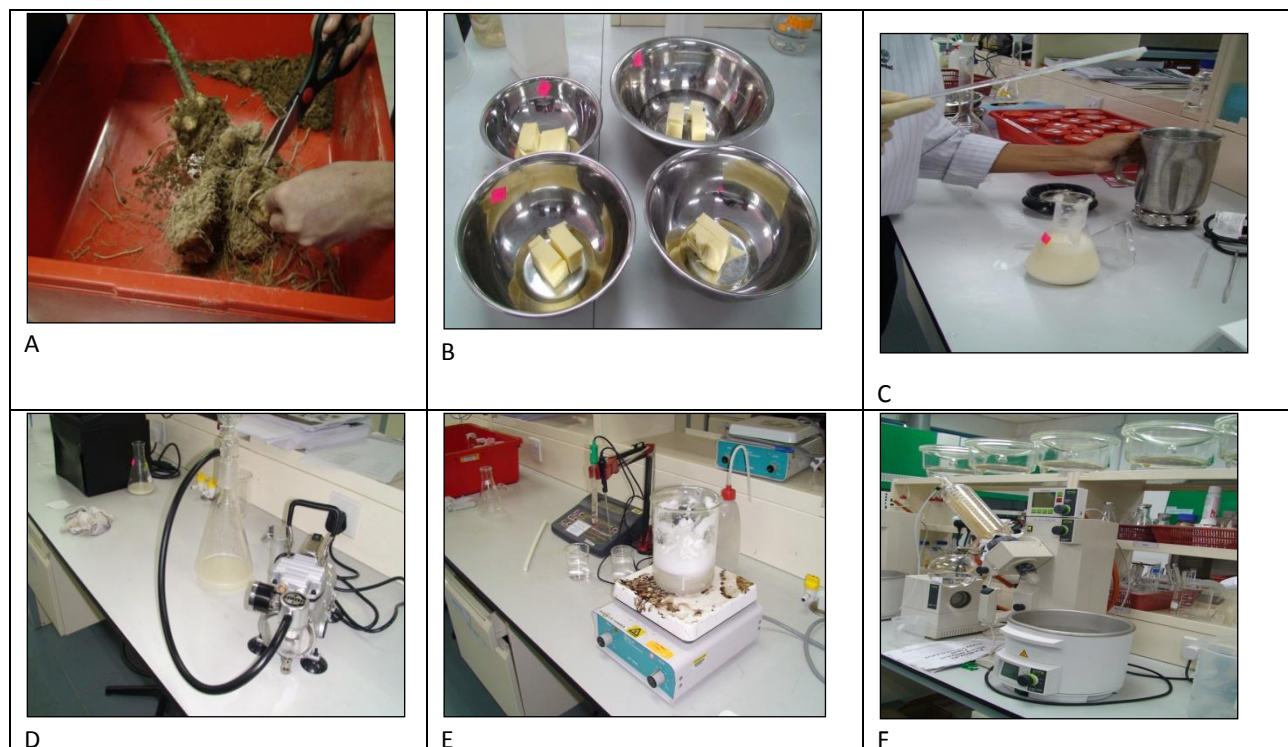
Fig. 3. The process flow for determination of alkaloid level in D. hispida ; A: cutting roots of rhizomes; B: slicing rhizomes ; C: blending with 200mL of 0.5M HCl ;D: filtering ; ; E: made alkaline of pH 10-11 ; F: concentrating under pressure by rotor evaporator.
